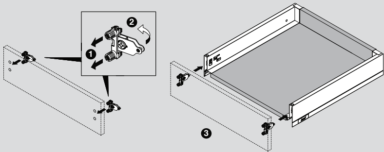
Standard Drawer K - Front Panel Assembly
