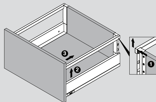
Standard Drawer HR Rectangular Rail - Removal
