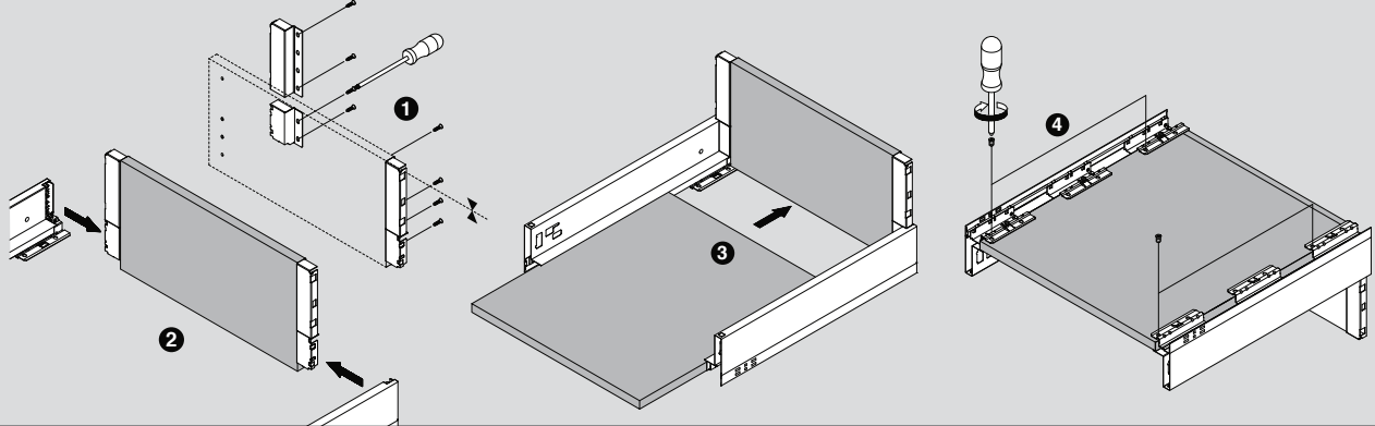
Standard Drawer S / T - Front Panel Assembly
