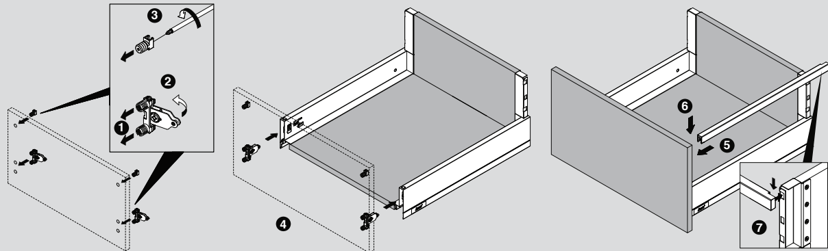
Internal Drawer S / T - Assembly
