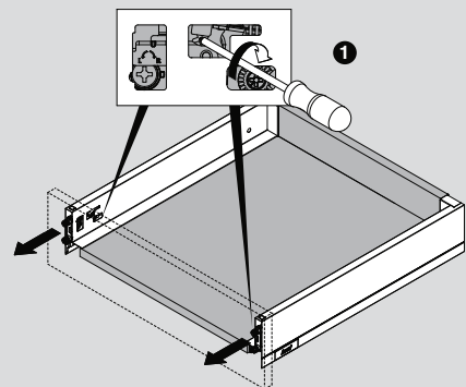
Standard Drawer K - Front Panel Removal
