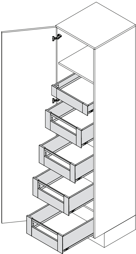
Pantry Kit with 1 x S Internal Drawer and 4 x K Internal Drawer
