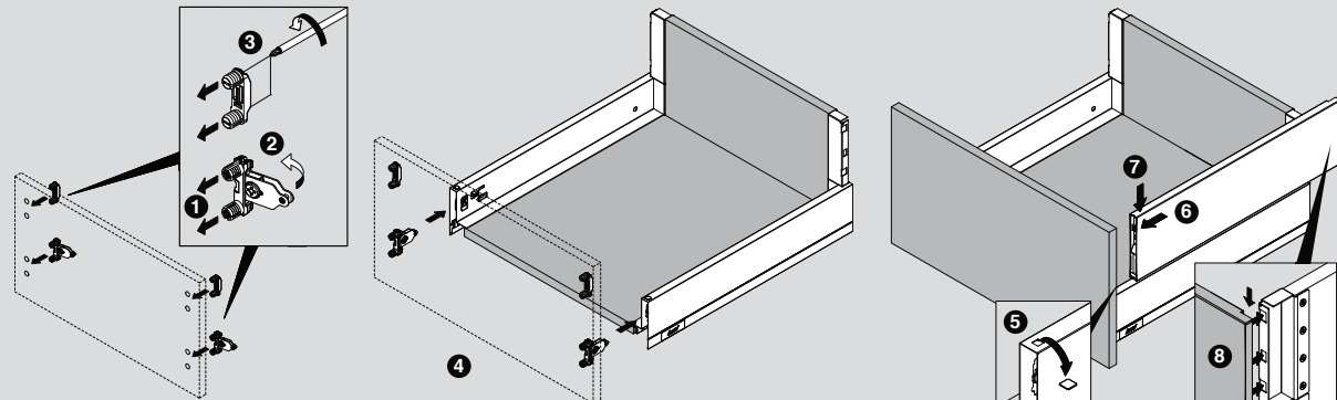
Standard Drawer HR Rectangular Rail - Front Panel and Railing Assembly
