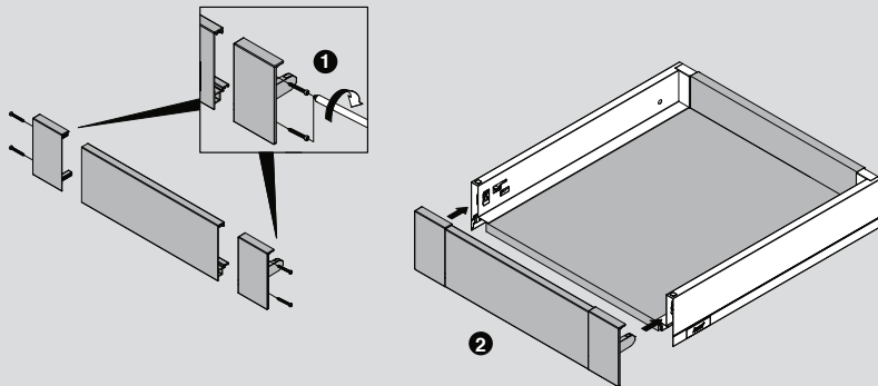
Internal Drawer K - Assembly
