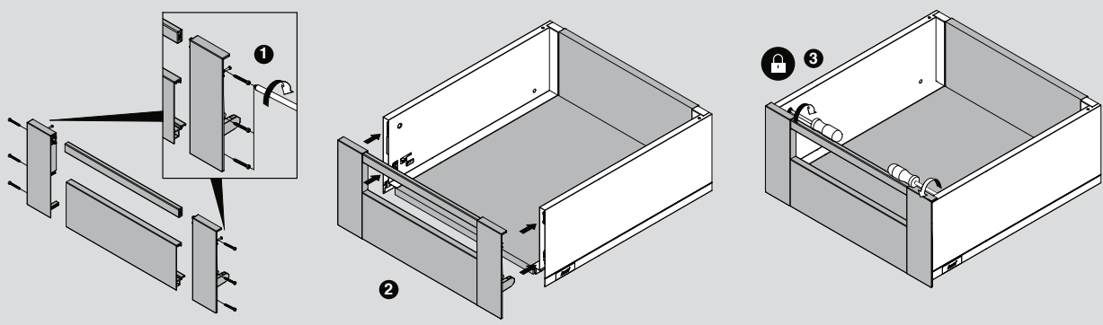
Internal Drawer K - Assembly
