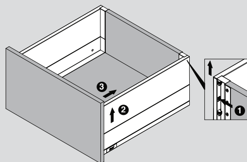
Standard Drawer HS / FS Side Extend - Removal
