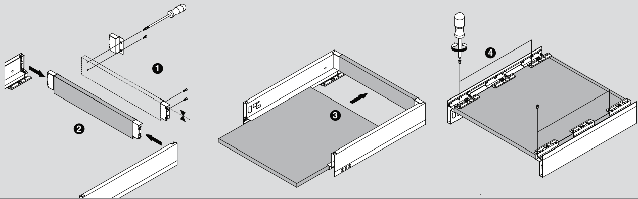
Standard Drawer HS / FS - Assembly
