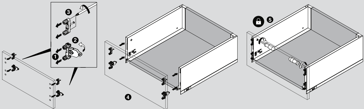
Standard Drawer K - Front Panel Assembly
