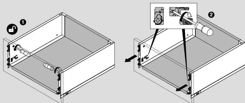
Standard Drawer HR Rectangular Rail - Removal
